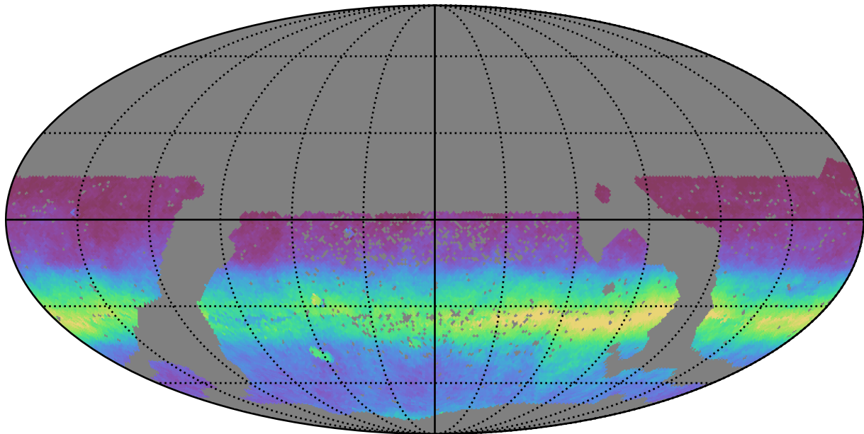
scp_reweight_v3.3_10yrs WFD all bands: AngleRms rotSkyPos
