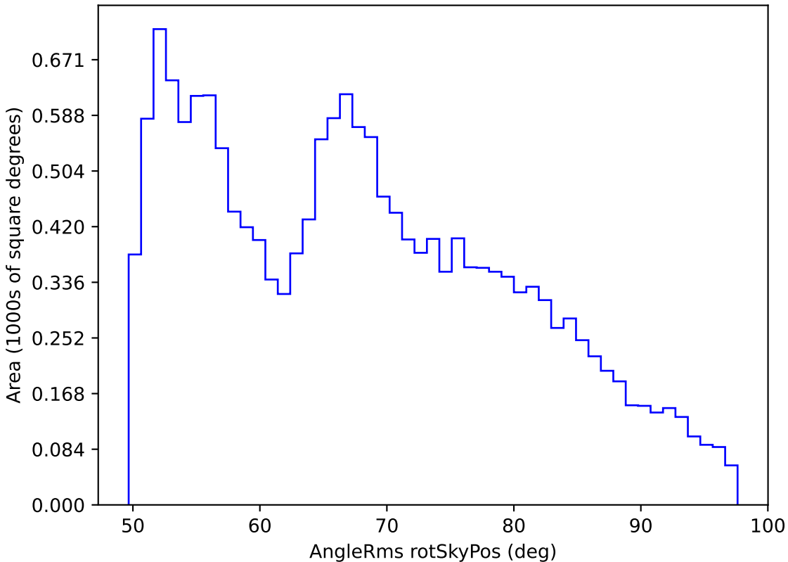
scp_reweight_v3.3_10yrs WFD all bands: AngleRms rotSkyPos
