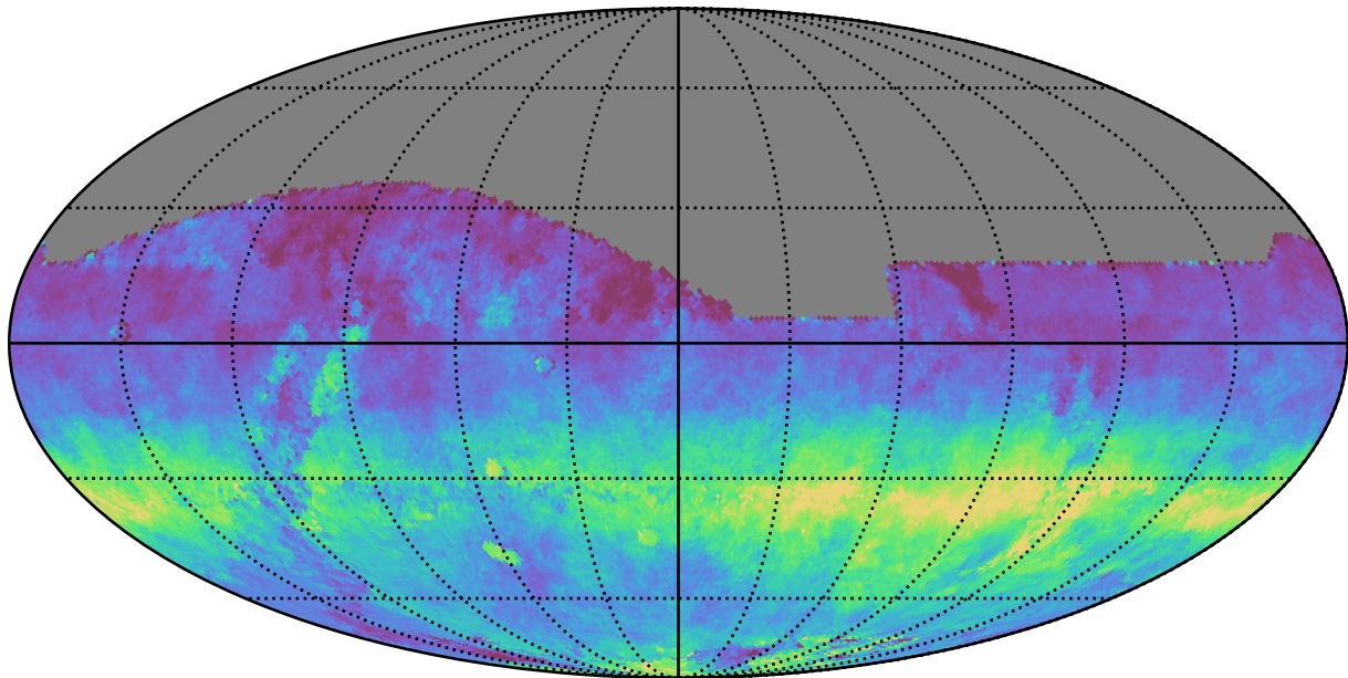
scp_reweight_v3.3_10yrs All sky z band: AngleRms rotSkyPos
