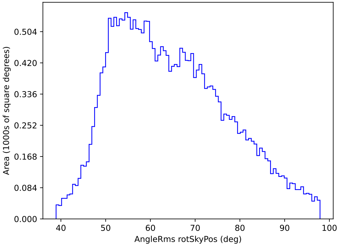
scp_reweight_v3.3_10yrs All sky z band: AngleRms rotSkyPos
