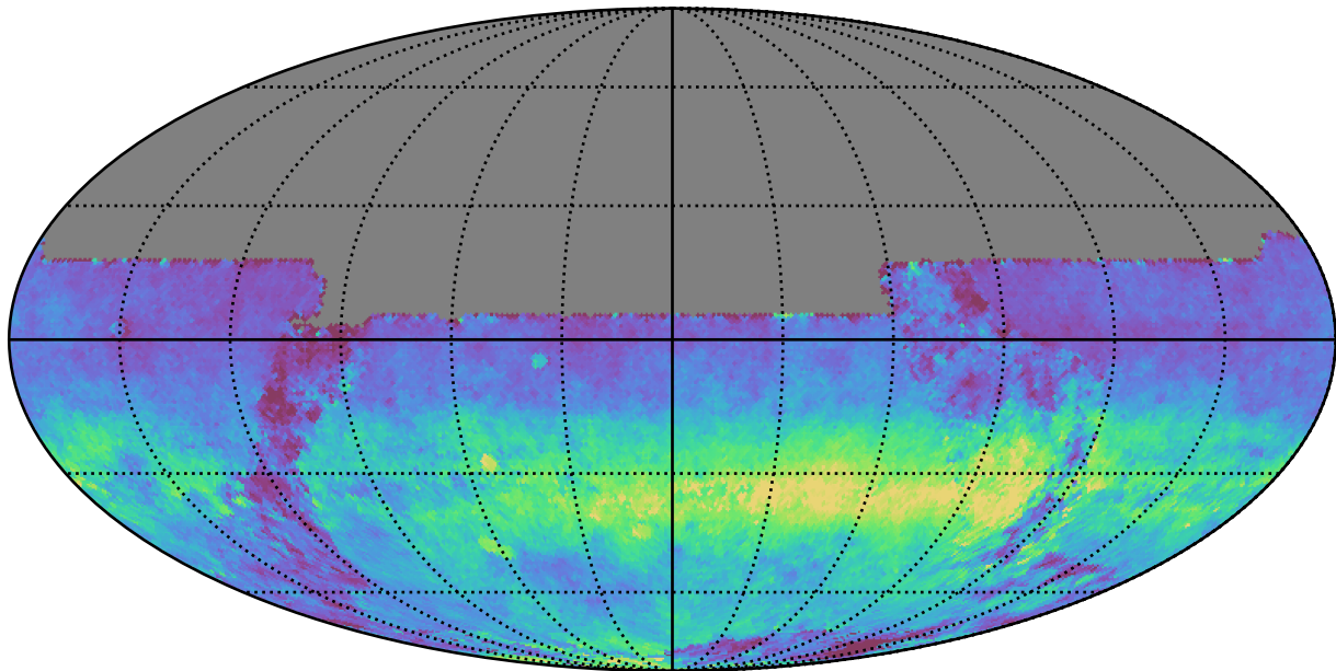
scp_reweight_v3.3_10yrs All sky y band: AngleRms rotSkyPos
