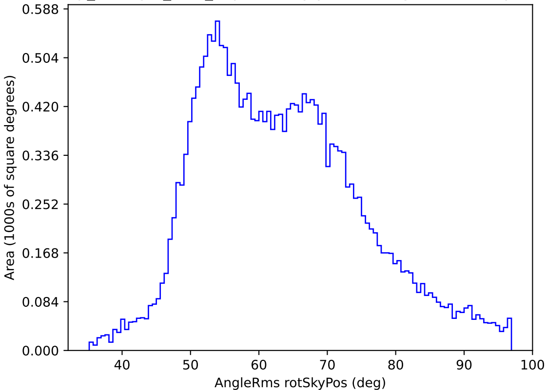
scp_reweight_v3.3_10yrs All sky y band: AngleRms rotSkyPos
