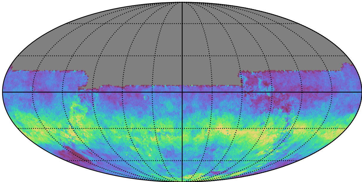
scp_reweight_v3.3_10yrs All sky u band: AngleRms rotSkyPos
