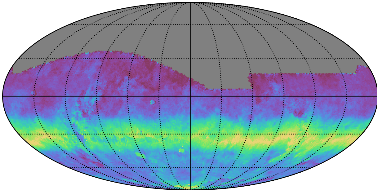
scp_reweight_v3.3_10yrs All sky r band: AngleRms rotSkyPos
