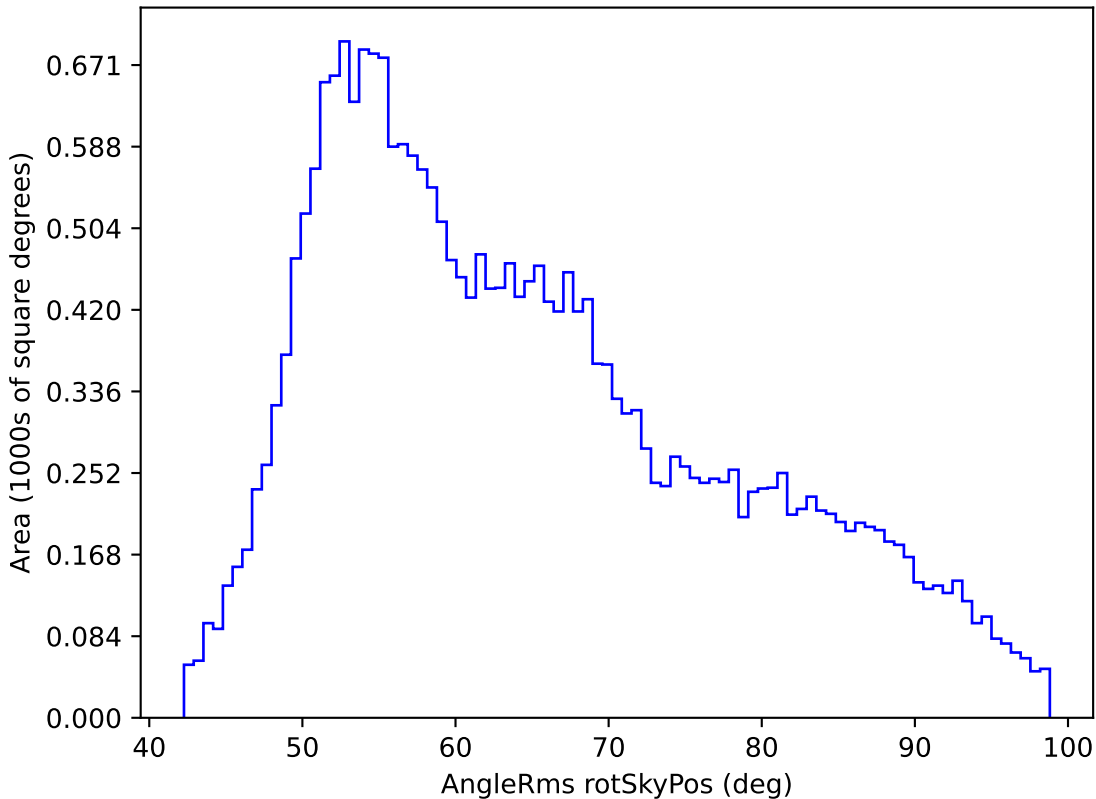
scp_reweight_v3.3_10yrs All sky r band: AngleRms rotSkyPos
