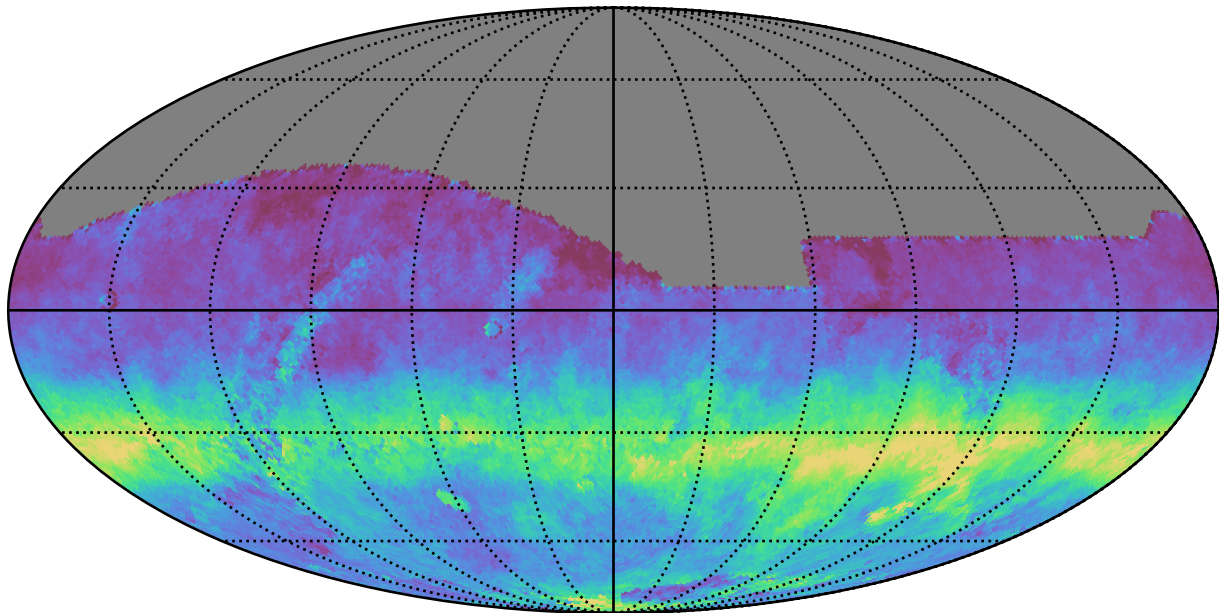
scp_reweight_v3.3_10yrs All sky i band: AngleRms rotSkyPos
