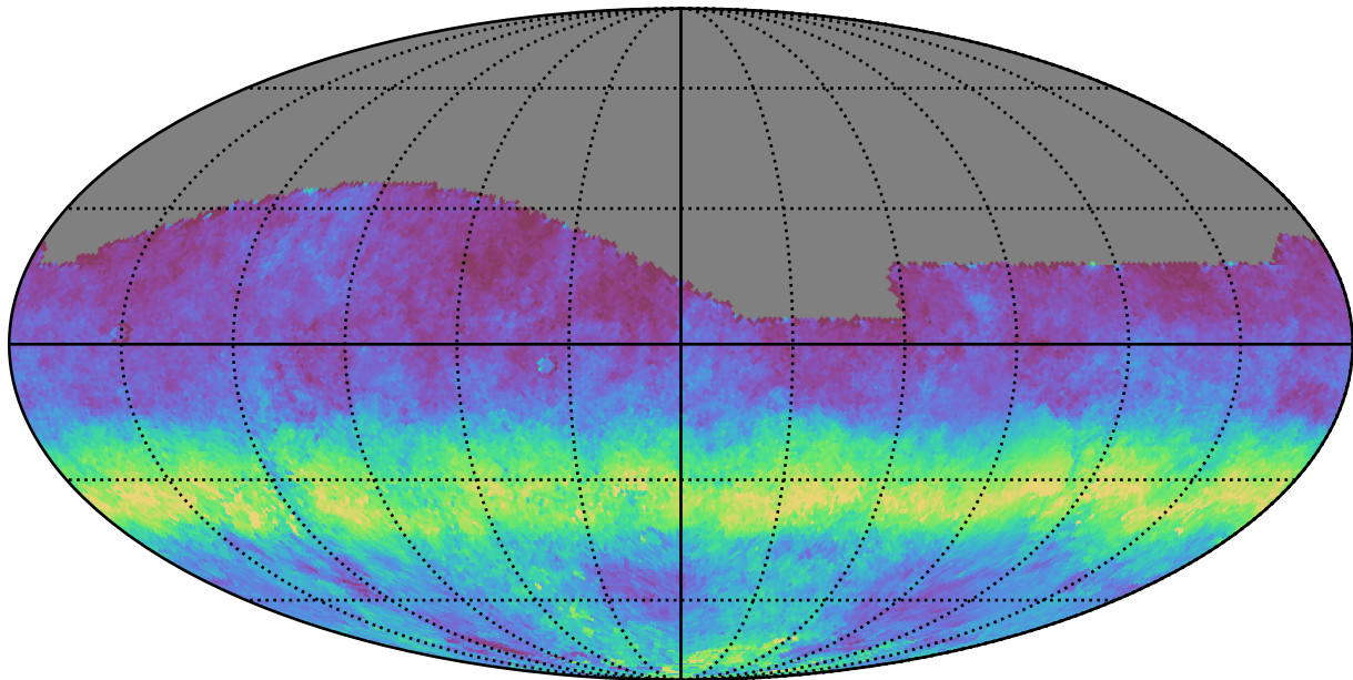
scp_reweight_v3.3_10yrs All sky g band: AngleRms rotSkyPos
