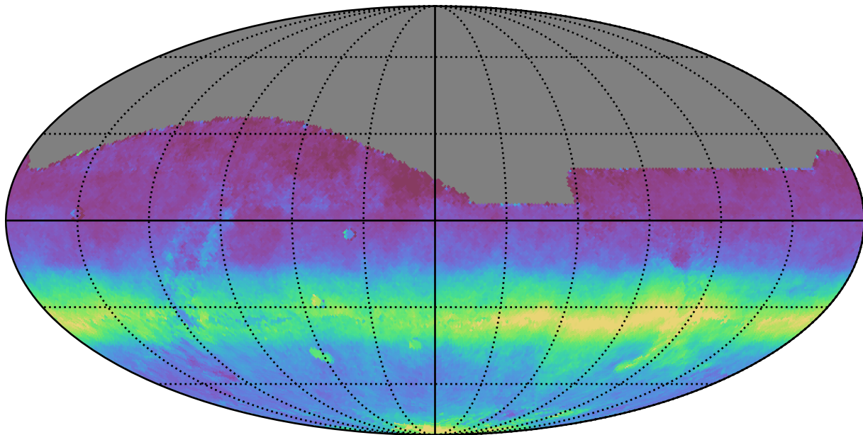
scp_reweight_v3.3_10yrs All sky all bands: AngleRms rotSkyPos
