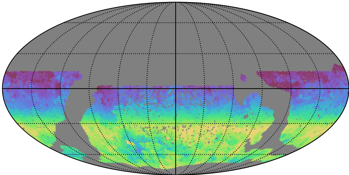
scp_reweight_v3.3_10yrs WFD z band: AngleRange rotSkyPos
