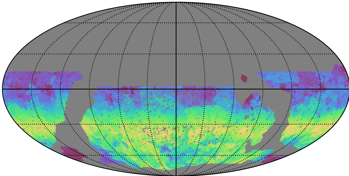
scp_reweight_v3.3_10yrs WFD u band: AngleRange rotSkyPos
