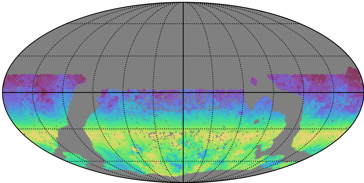
scp_reweight_v3.3_10yrs WFD r band: AngleRange rotSkyPos
