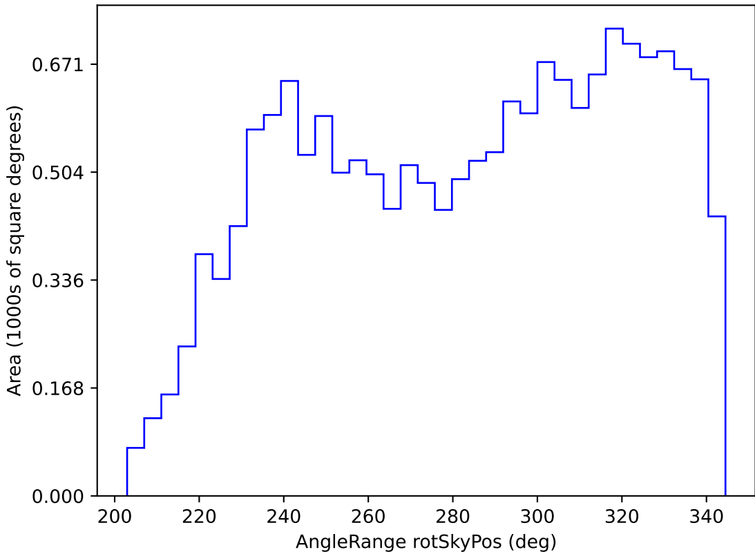
scp_reweight_v3.3_10yrs WFD r band: AngleRange rotSkyPos
