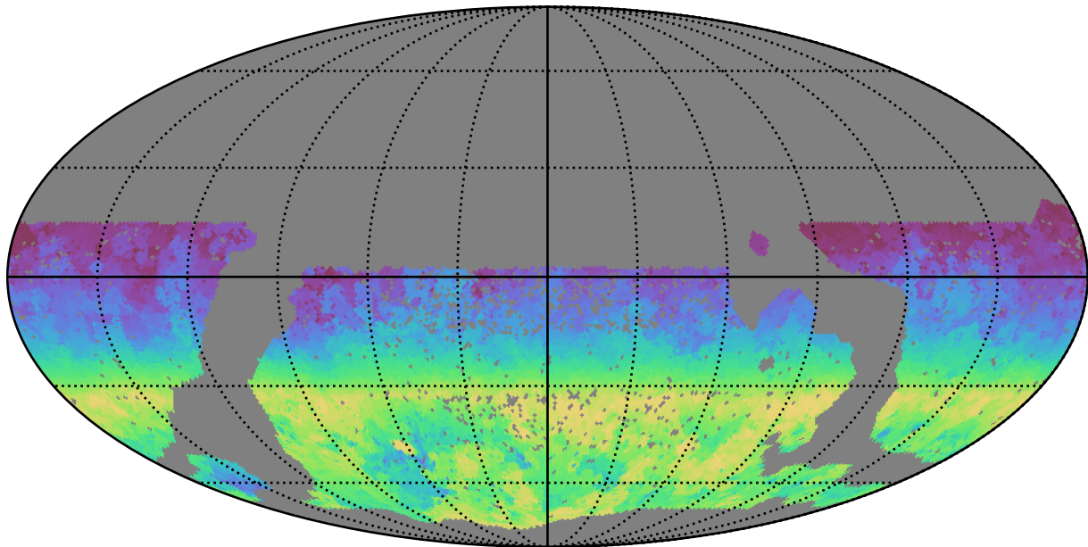
scp_reweight_v3.3_10yrs WFD i band: AngleRange rotSkyPos
