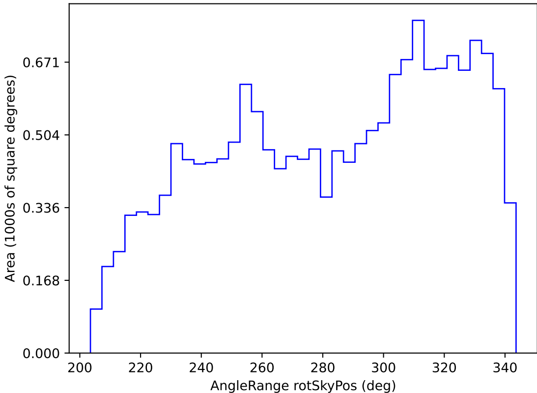
scp_reweight_v3.3_10yrs WFD i band: AngleRange rotSkyPos
