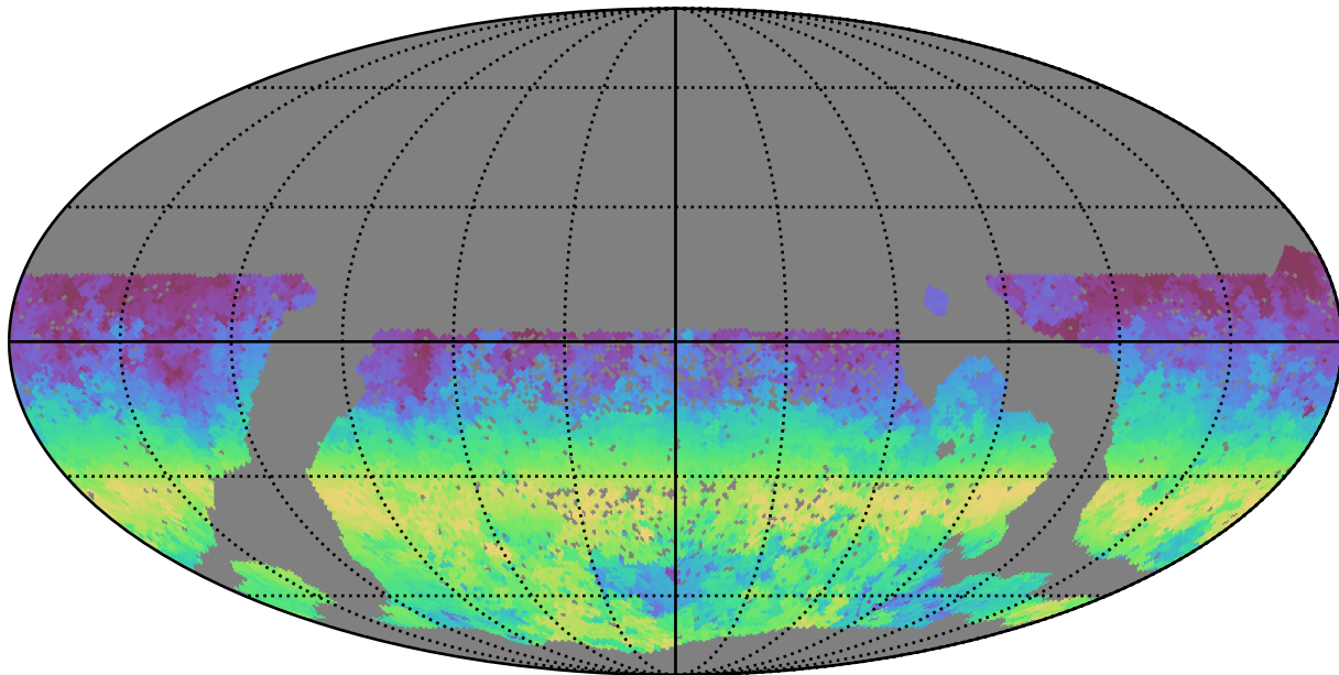
scp_reweight_v3.3_10yrs WFD g band: AngleRange rotSkyPos
