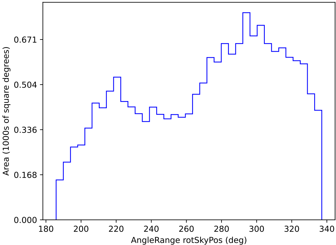
scp_reweight_v3.3_10yrs WFD g band: AngleRange rotSkyPos
