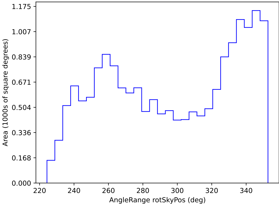
scp_reweight_v3.3_10yrs WFD all bands: AngleRange rotSkyPos
