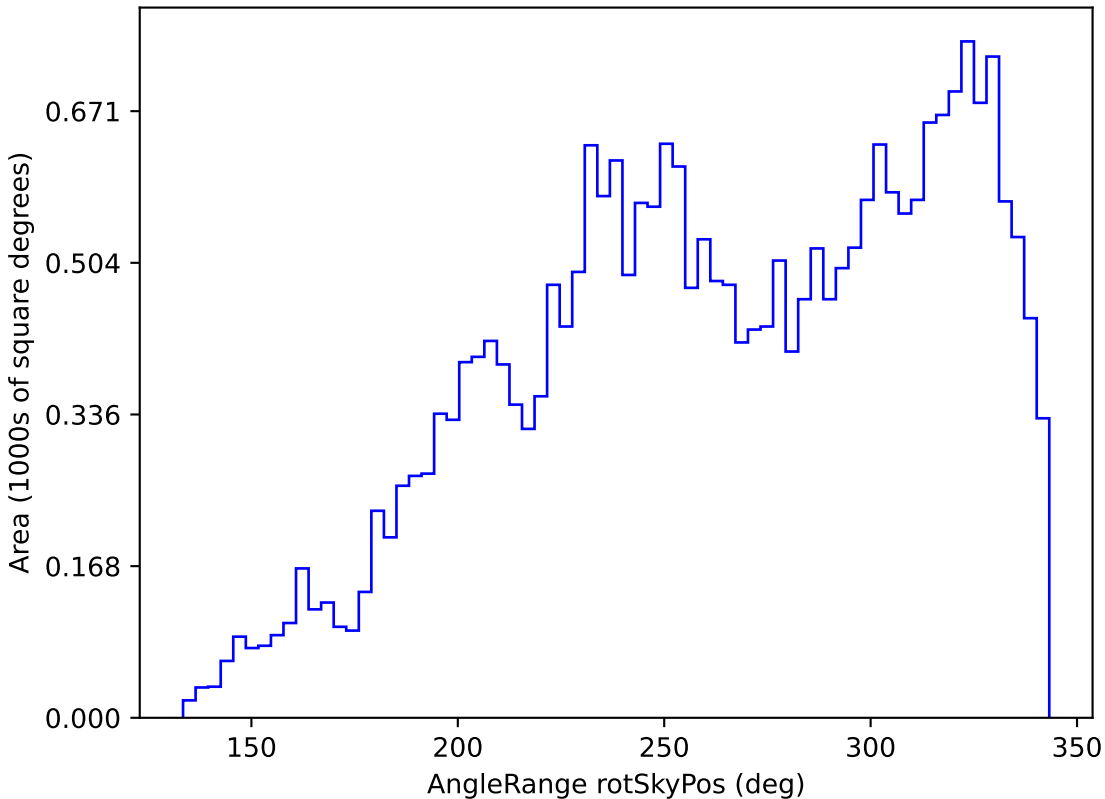
scp_reweight_v3.3_10yrs All sky z band: AngleRange rotSkyPos
