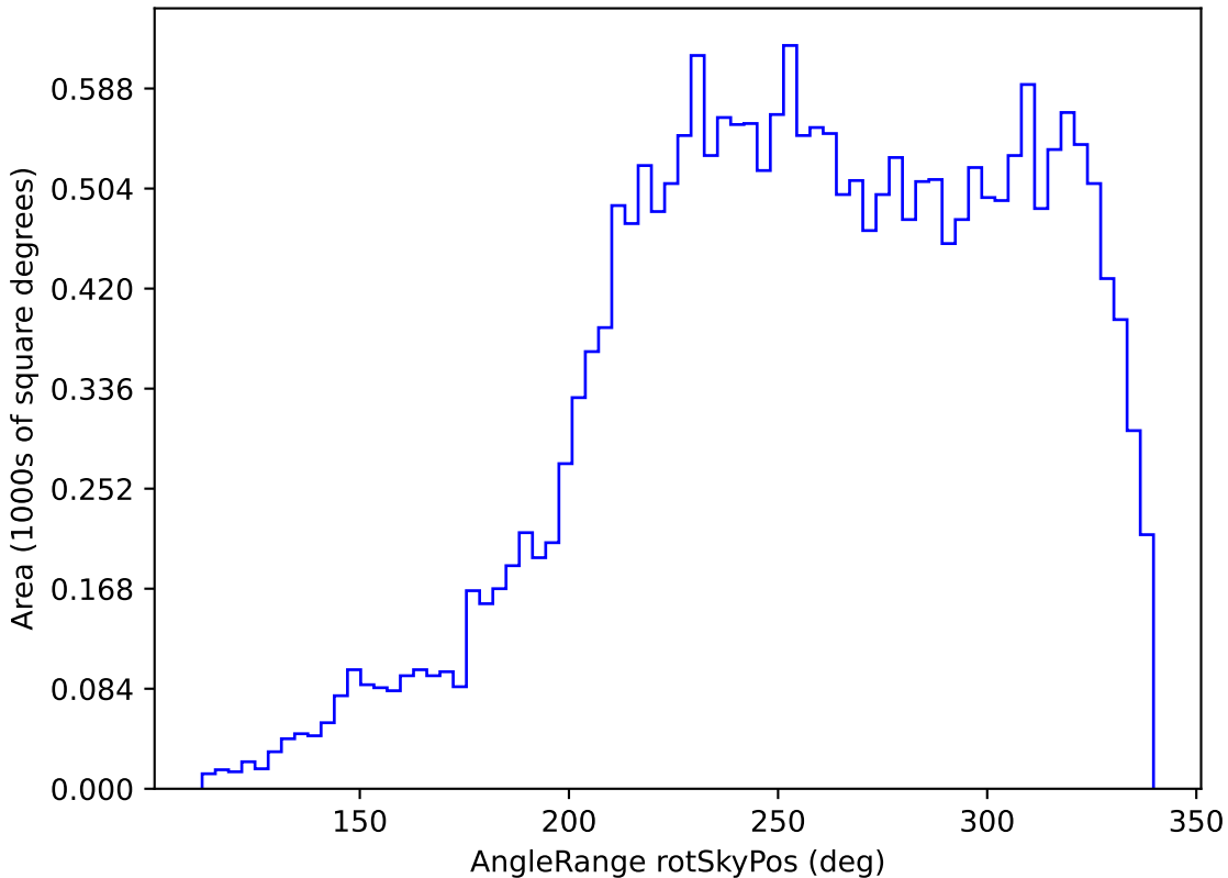
scp_reweight_v3.3_10yrs All sky y band: AngleRange rotSkyPos
