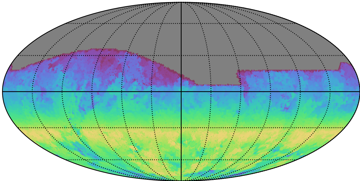
scp_reweight_v3.3_10yrs All sky r band: AngleRange rotSkyPos
