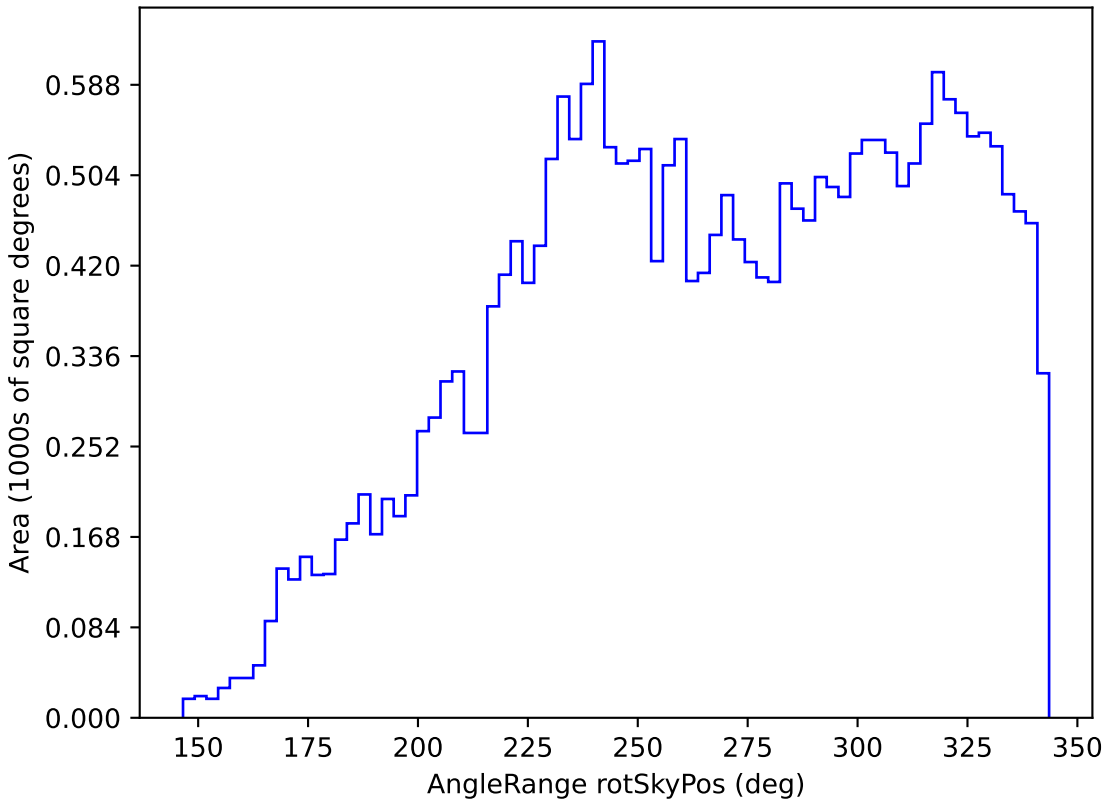
scp_reweight_v3.3_10yrs All sky r band: AngleRange rotSkyPos
