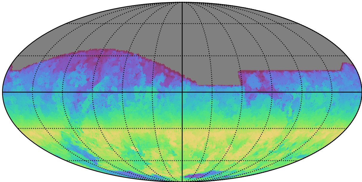
scp_reweight_v3.3_10yrs All sky i band: AngleRange rotSkyPos
