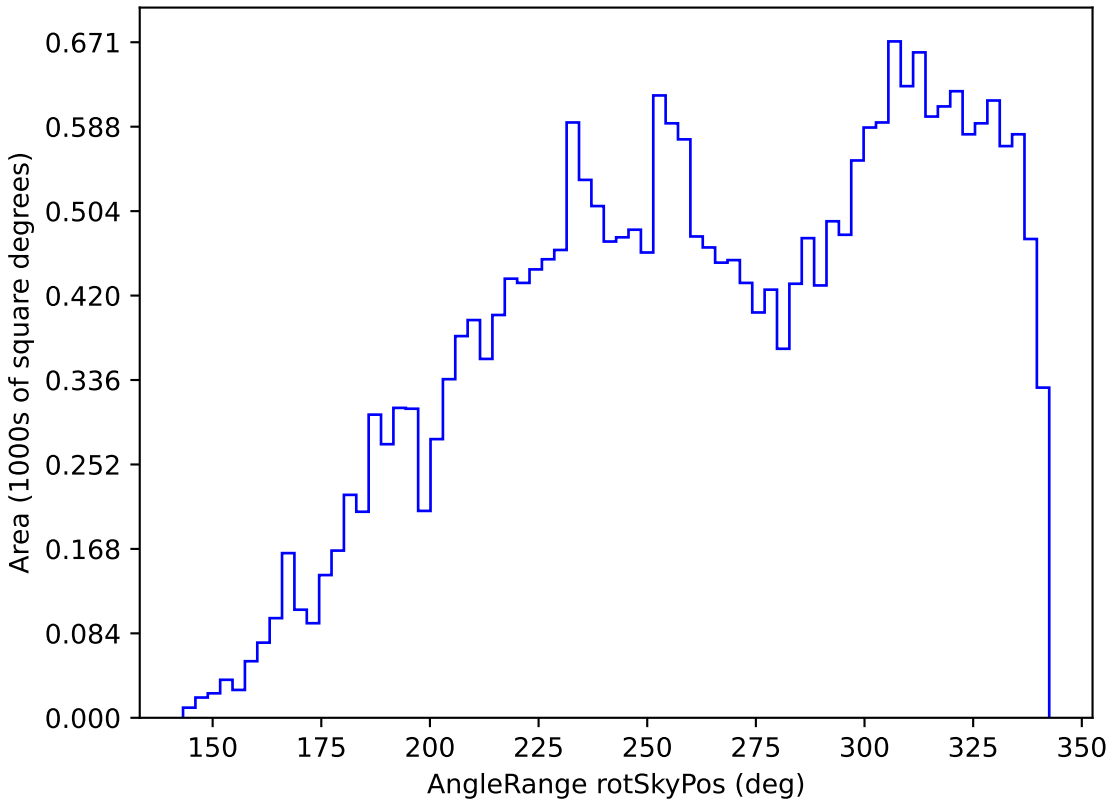
scp_reweight_v3.3_10yrs All sky i band: AngleRange rotSkyPos
