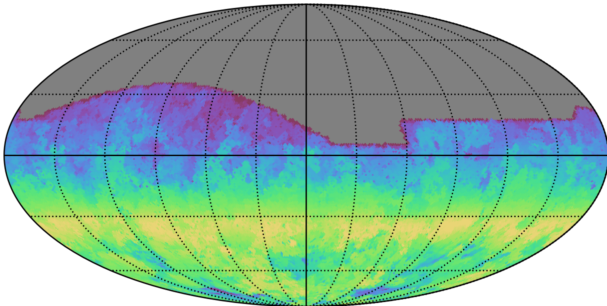
scp_reweight_v3.3_10yrs All sky g band: AngleRange rotSkyPos
