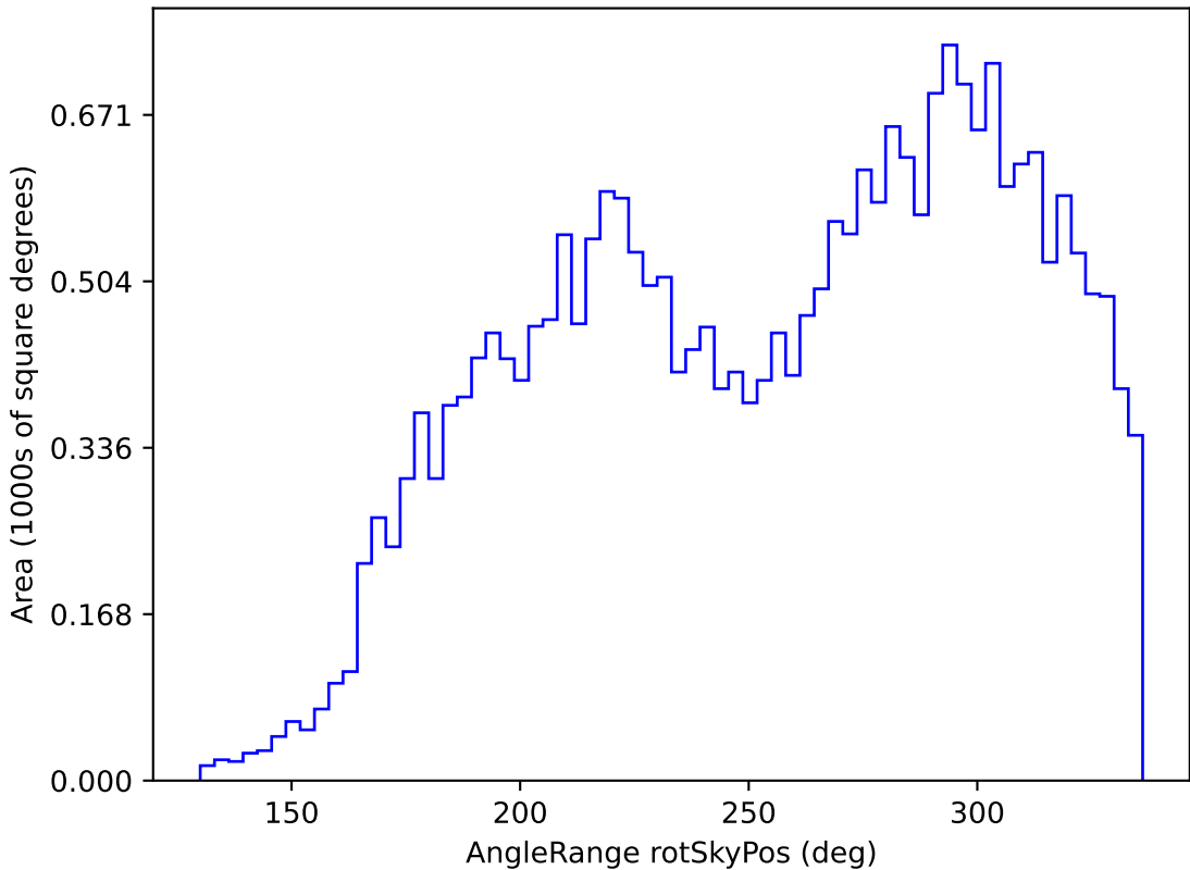
scp_reweight_v3.3_10yrs All sky g band: AngleRange rotSkyPos
