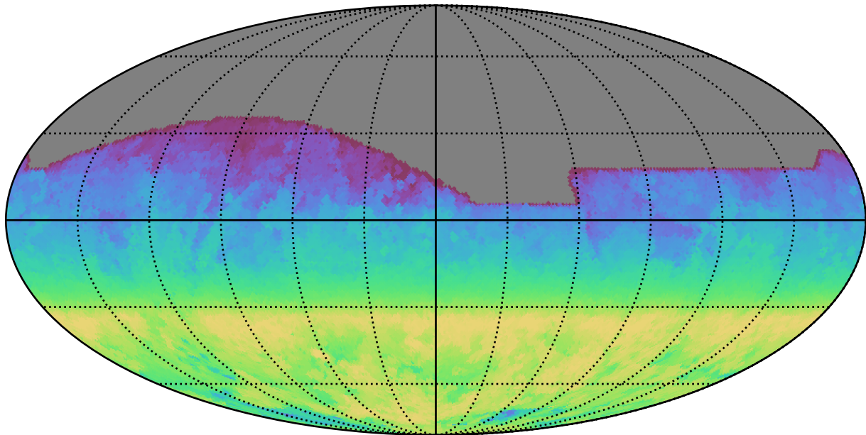
scp_reweight_v3.3_10yrs All sky all bands: AngleRange rotSkyPos
