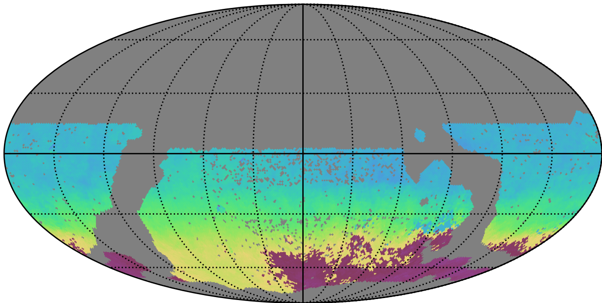
scp_reweight_v3.3_10yrs WFD z band: AngleMean rotSkyPos
