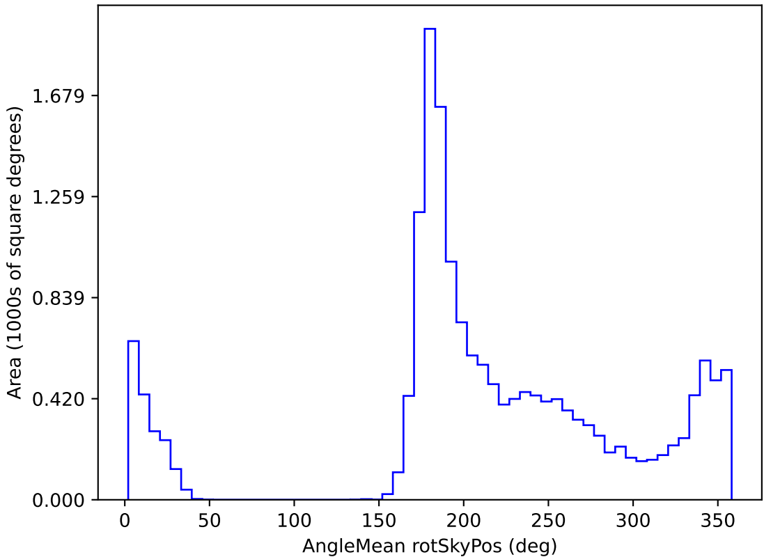
scp_reweight_v3.3_10yrs WFD z band: AngleMean rotSkyPos
