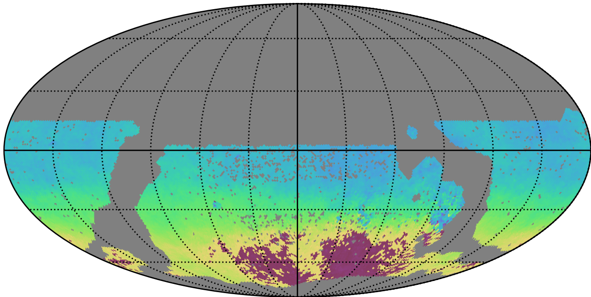
scp_reweight_v3.3_10yrs WFD y band: AngleMean rotSkyPos
