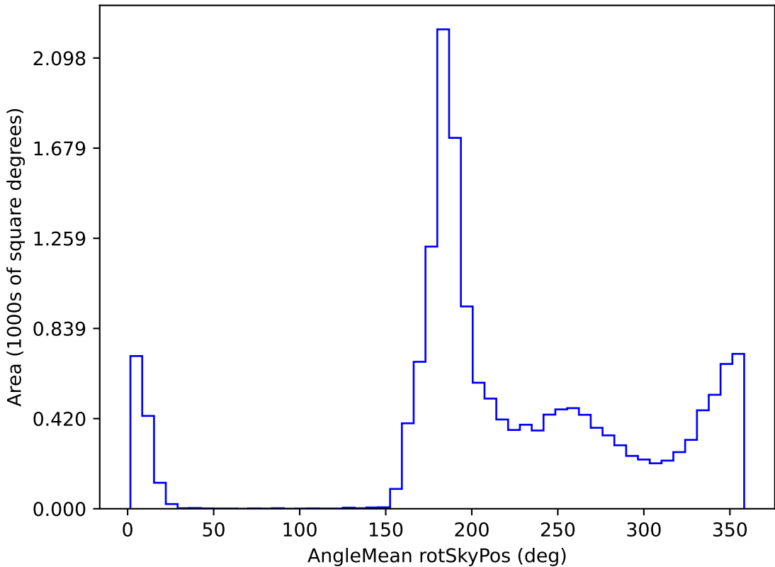
scp_reweight_v3.3_10yrs WFD y band: AngleMean rotSkyPos
