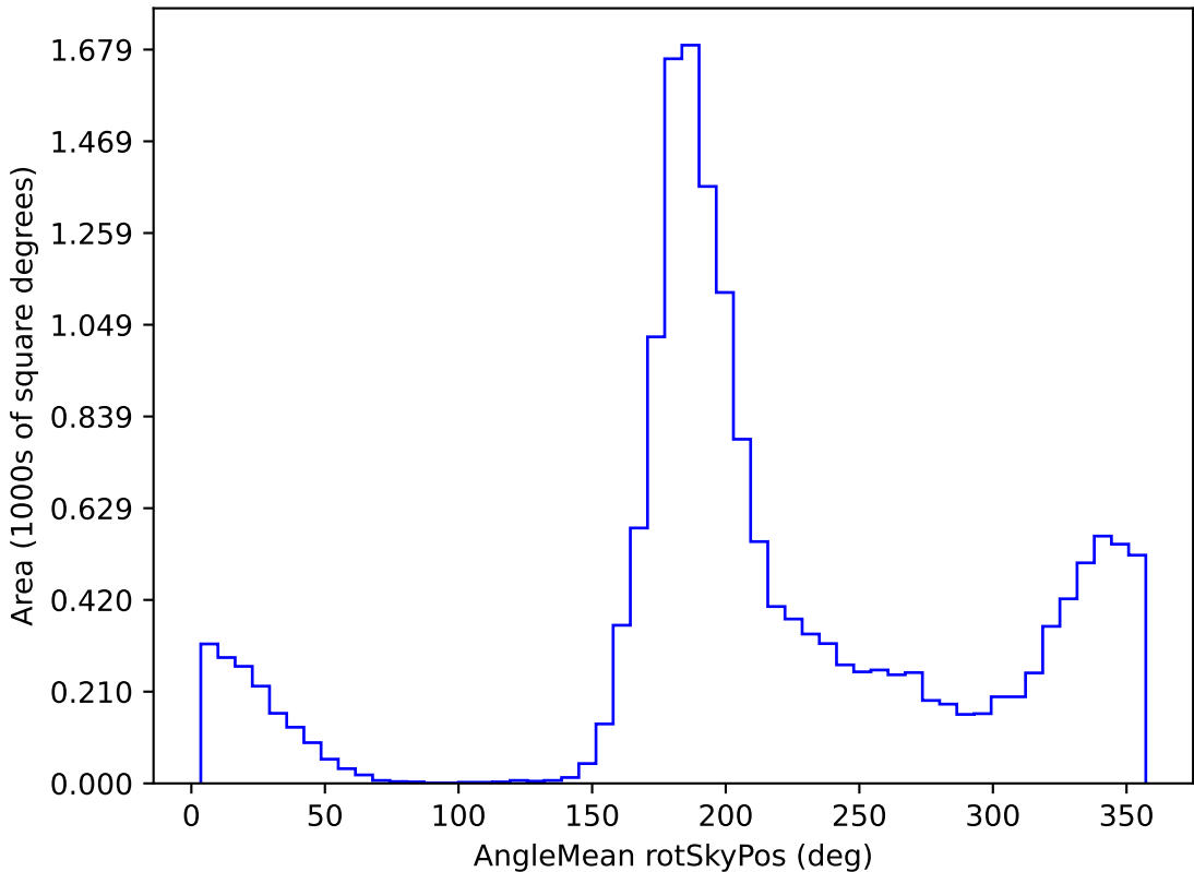
scp_reweight_v3.3_10yrs WFD u band: AngleMean rotSkyPos
