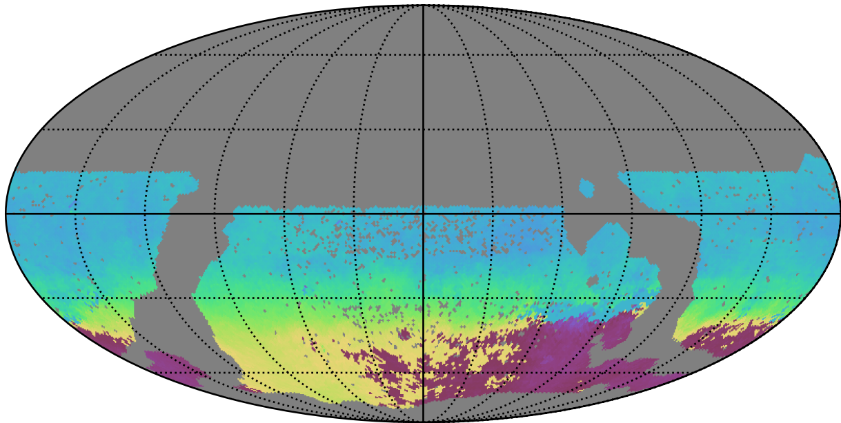
scp_reweight_v3.3_10yrs WFD r band: AngleMean rotSkyPos
