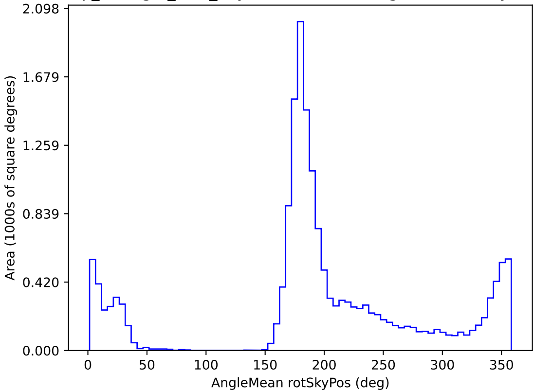
scp_reweight_v3.3_10yrs WFD r band: AngleMean rotSkyPos
