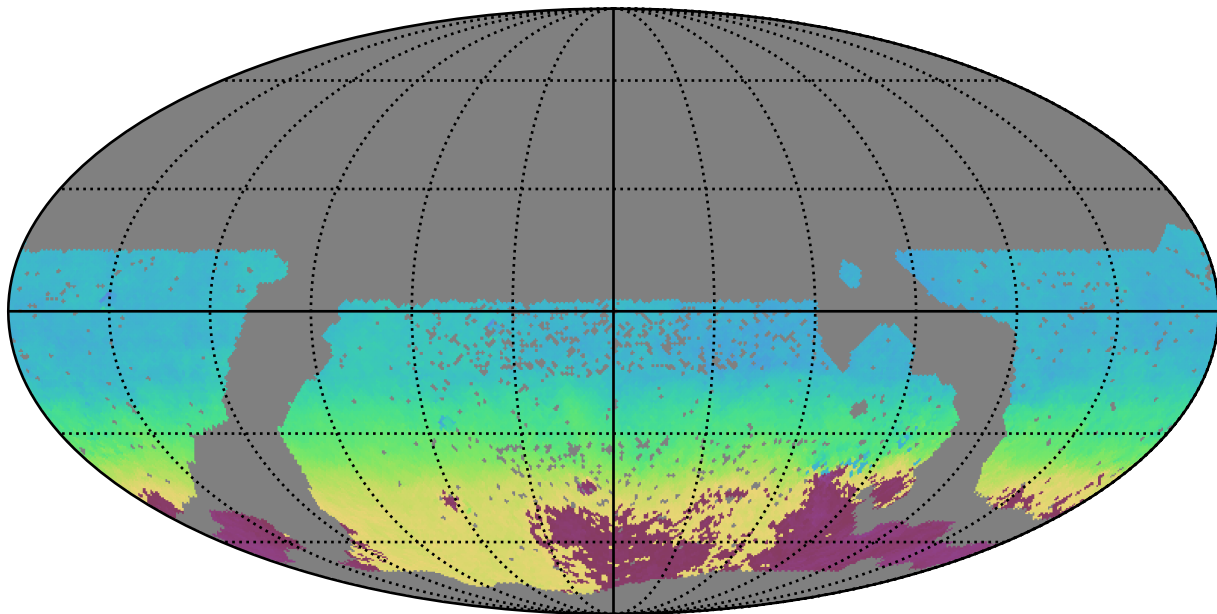
scp_reweight_v3.3_10yrs WFD i band: AngleMean rotSkyPos
