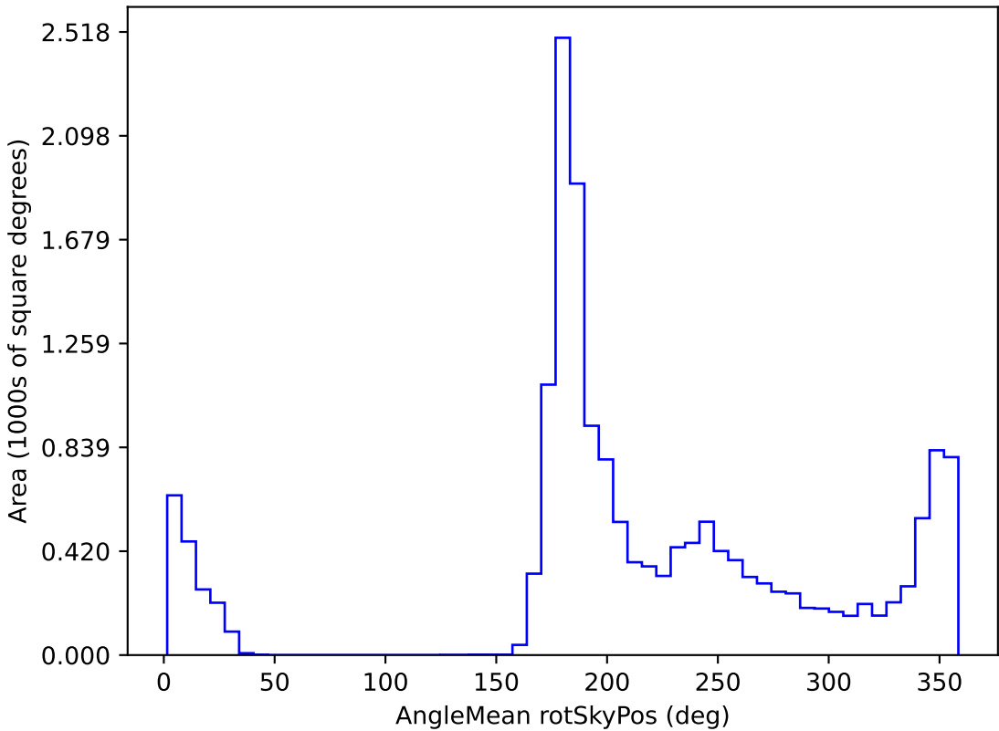
scp_reweight_v3.3_10yrs WFD i band: AngleMean rotSkyPos
