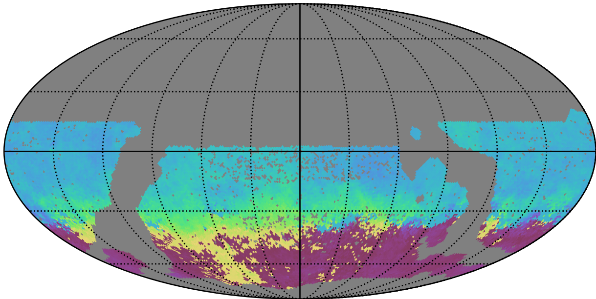
scp_reweight_v3.3_10yrs WFD g band: AngleMean rotSkyPos
