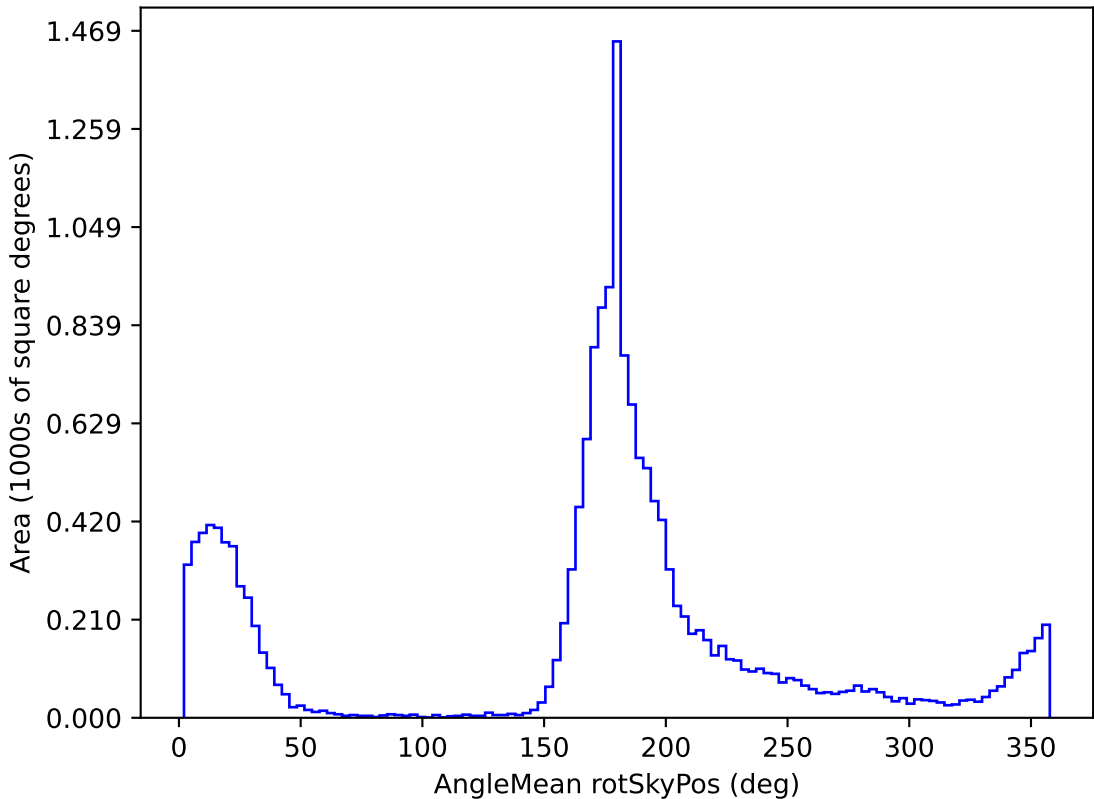
scp_reweight_v3.3_10yrs WFD g band: AngleMean rotSkyPos
