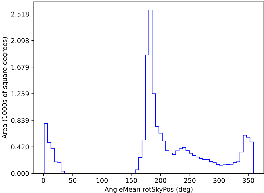
scp_reweight_v3.3_10yrs WFD all bands: AngleMean rotSkyPos
