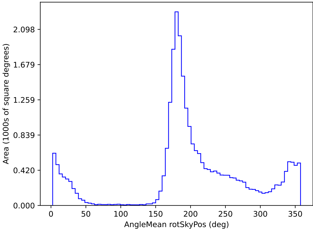
scp_reweight_v3.3_10yrs All sky z band: AngleMean rotSkyPos
