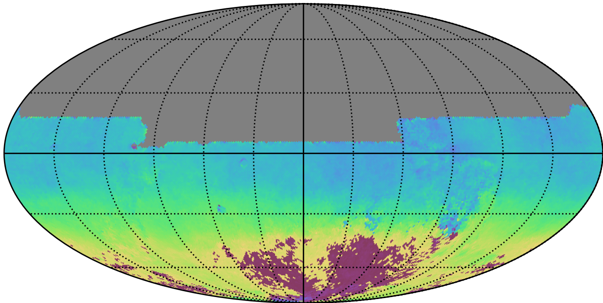
scp_reweight_v3.3_10yrs All sky y band: AngleMean rotSkyPos
