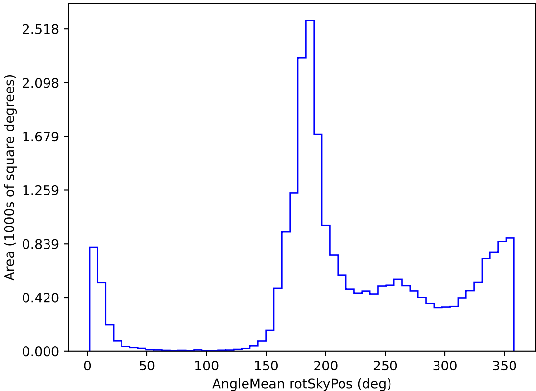
scp_reweight_v3.3_10yrs All sky y band: AngleMean rotSkyPos
