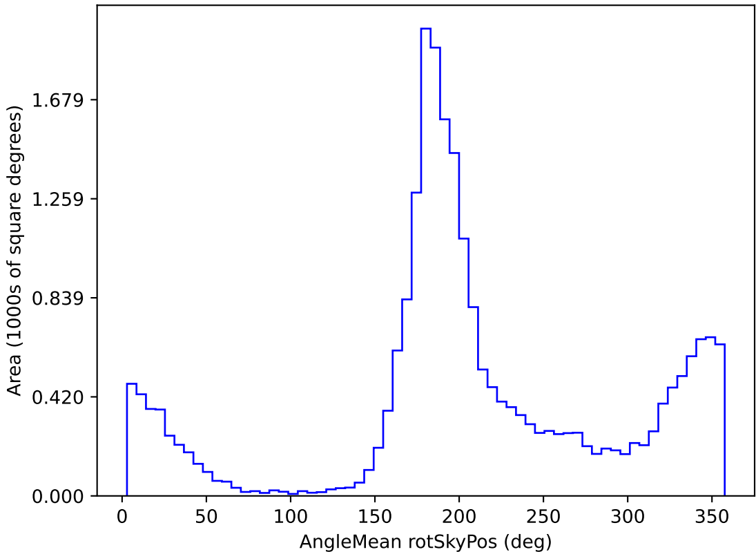
scp_reweight_v3.3_10yrs All sky u band: AngleMean rotSkyPos
