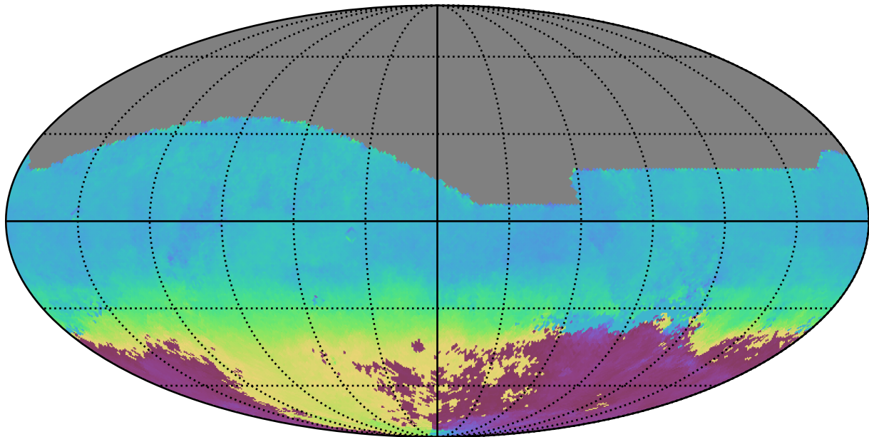
scp_reweight_v3.3_10yrs All sky r band: AngleMean rotSkyPos
