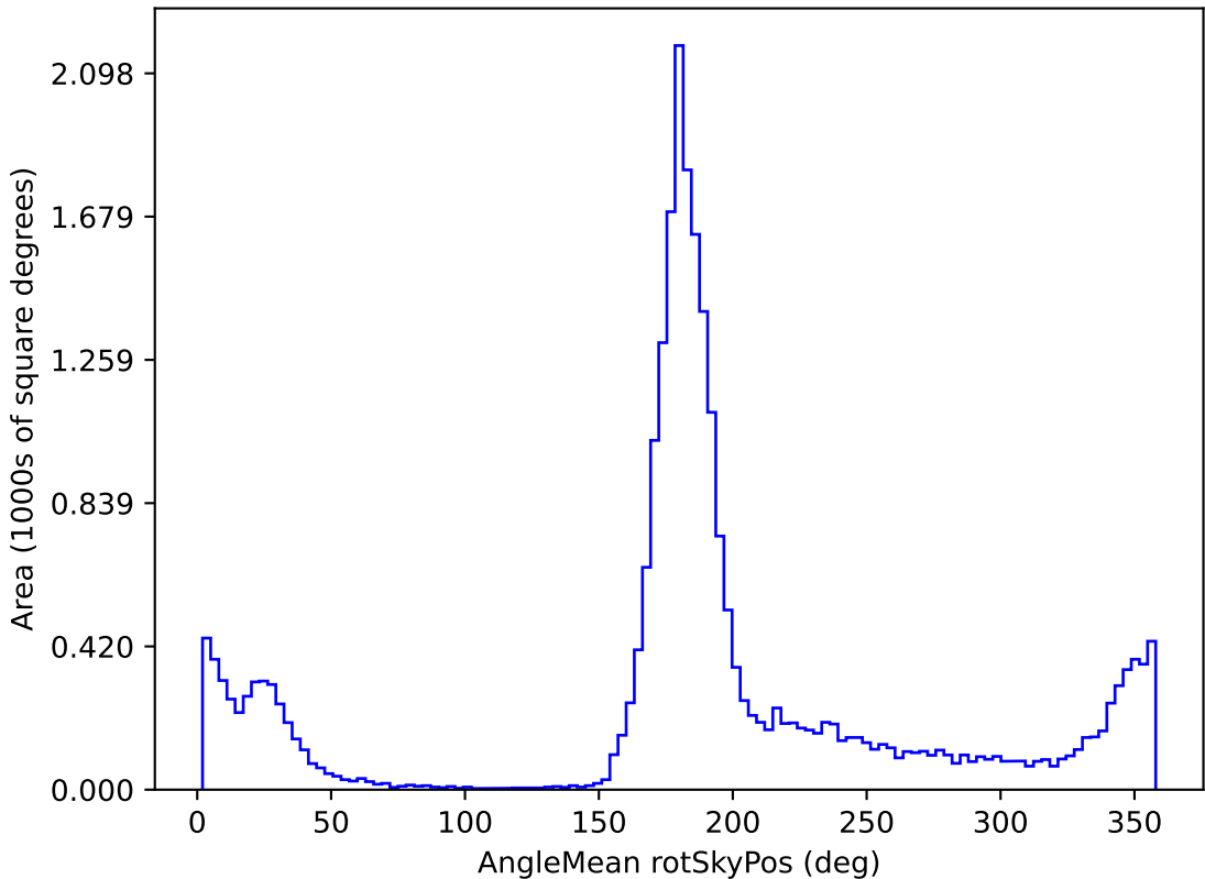
scp_reweight_v3.3_10yrs All sky r band: AngleMean rotSkyPos
