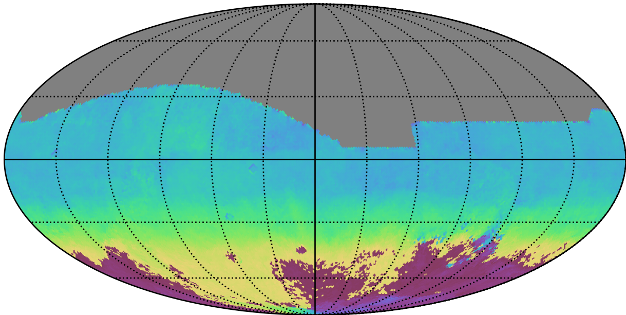
scp_reweight_v3.3_10yrs All sky i band: AngleMean rotSkyPos
