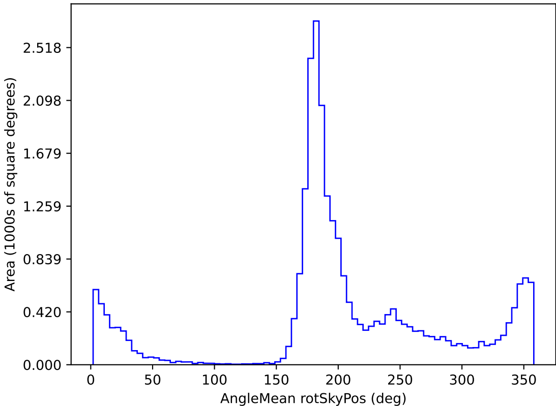
scp_reweight_v3.3_10yrs All sky i band: AngleMean rotSkyPos
